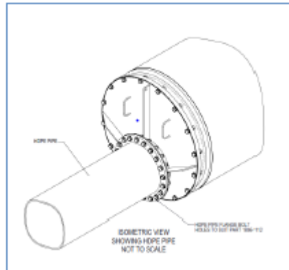
Fig 4. Steel flange and PE pipe connected
