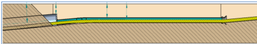
Fig 5. PE pipe with power cable inside on seabed.
