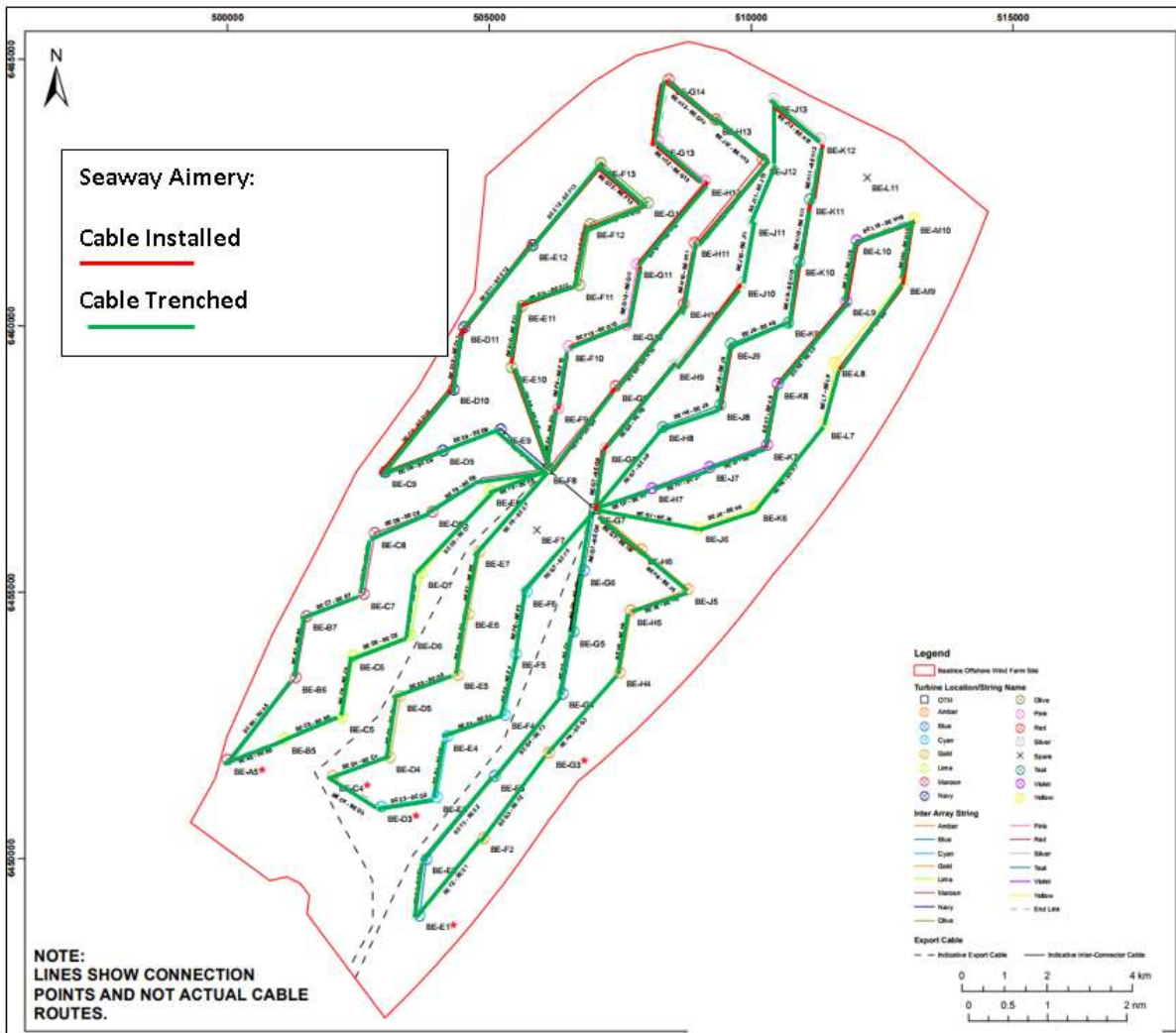
Fig. 2 Cable Installation Progress
